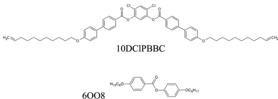
Figure 1. Structural formulas of the bent-core 10DCIPBBC and the rod-shaped 6OO8 molecules used in the experiment.
