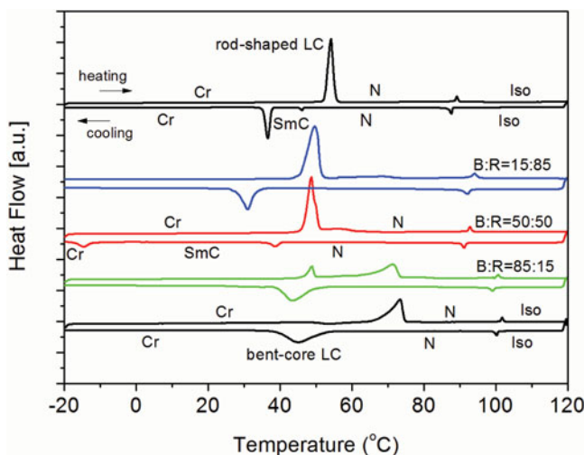
Figure 2. DSC thermograms obtained for the bent-core (B) and the rod-shaped (R) LCs and for their mixtures with different weight ratios B:R during the first heating and cooling cycle at the rate of 10°C/min.
