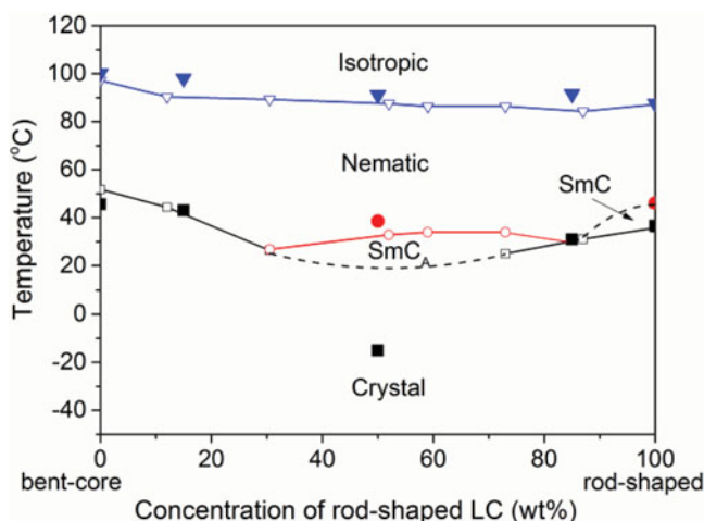
Figure 3. The phase diagram of the binary mixtures of the bent-core and rod-shaped compounds (solid symbols correspond to our DSC measurements at cooling, open symbols indicate the results of the polarizing microscope measurements in [10]).
