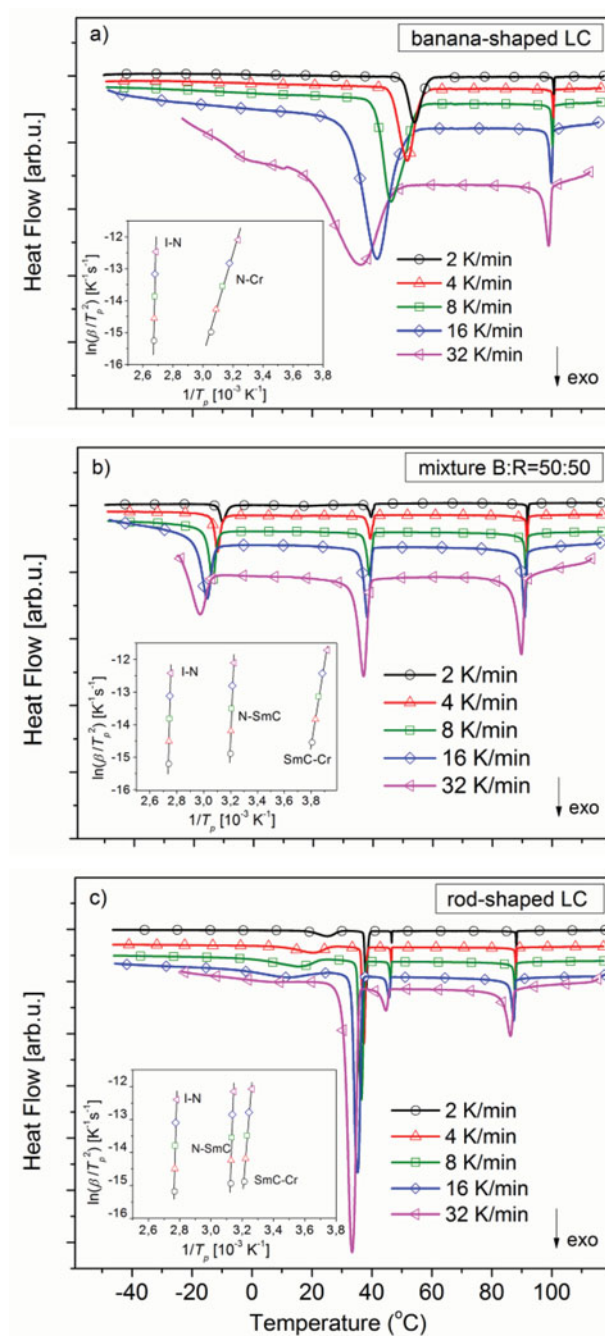
Figure 4. DSC traces obtained during cooling for the samples of a) the pure banana-shaped LC, b) the mixture of banana and rod-shaped LCs with 50:50 weight ratio and c) the pure rod-shaped LC. Insets show the corresponding Kissinger plots for the individual phase transition peaks.
